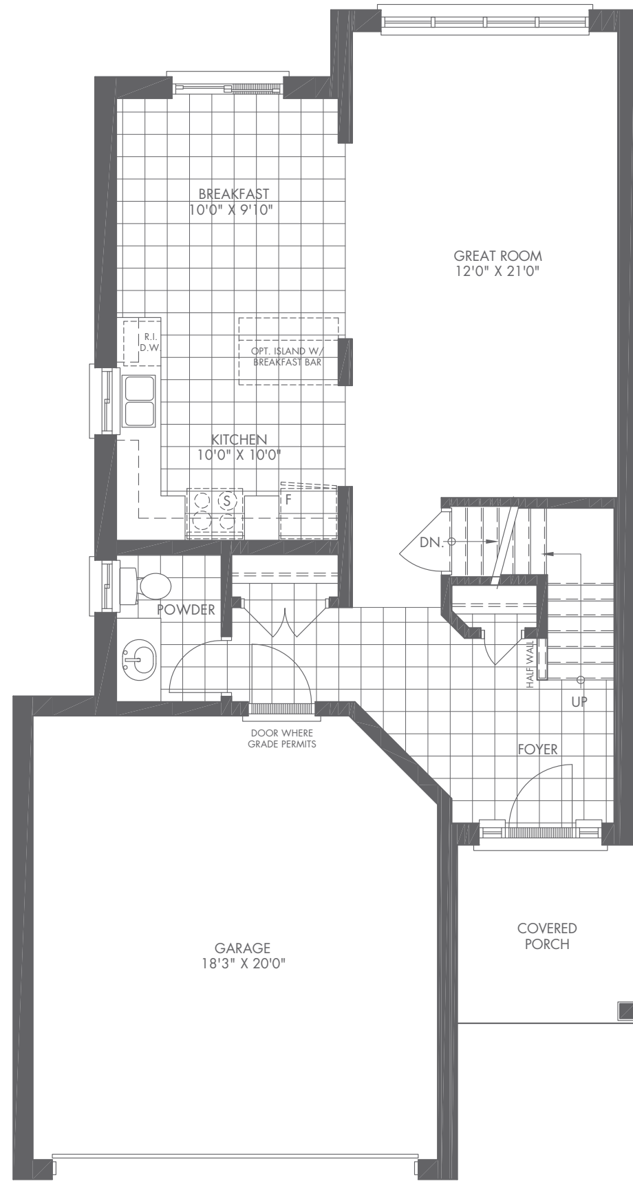
GROUND FLOOR ELEV. A & B
