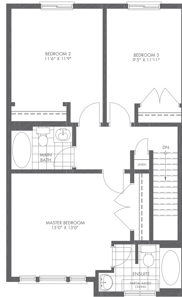
2ND FLOOR ELEV. A
