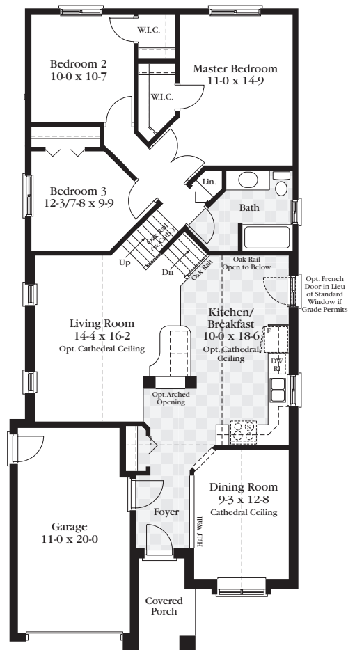
OPTIONAL UPPER AND LOWER FLOOR PLAN
