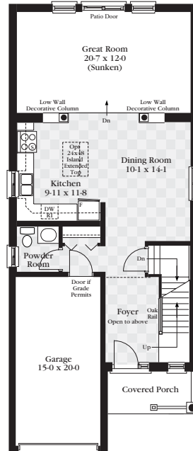
Main Floor Plan Elevation C
